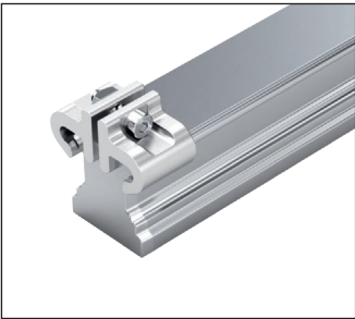
Ball guide rails with cover strip and strip clamps made of aluminum
