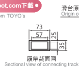
滑台原點148.5±1 Origin of actuator:148.5±1
